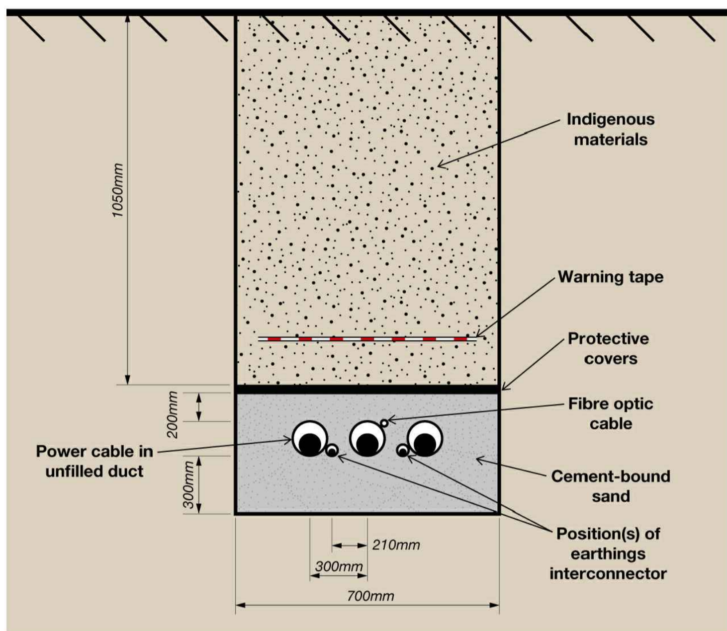
Typical Underground HVAC Arrangement
